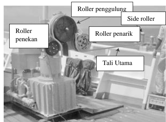
Gambar 17 Line hauler
